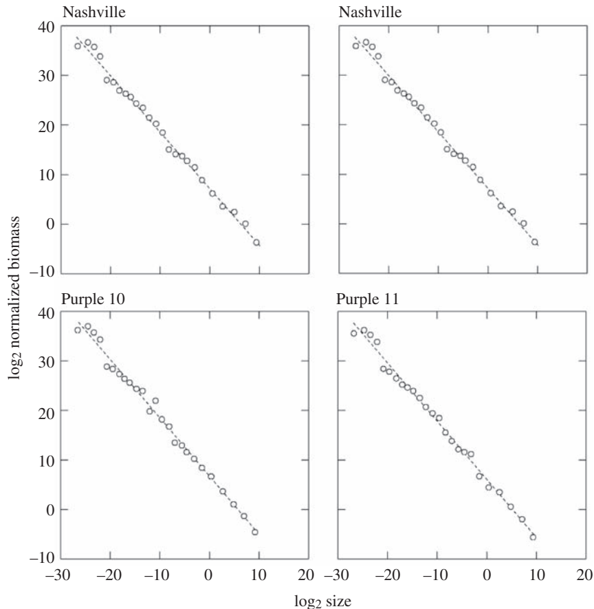
Fig. 7. Normalized biomass size-spectra in carbon units from several stations in the New England Seamounts Area (Northwest Atlantic). Size range: 1.6 \times 10^{-9} to 1.33 \times 10^3 g C individual -1 (from bacteria to meso-zooplankton). Depth range: 0–400 m. (After Quiñones et al., 2003.)
